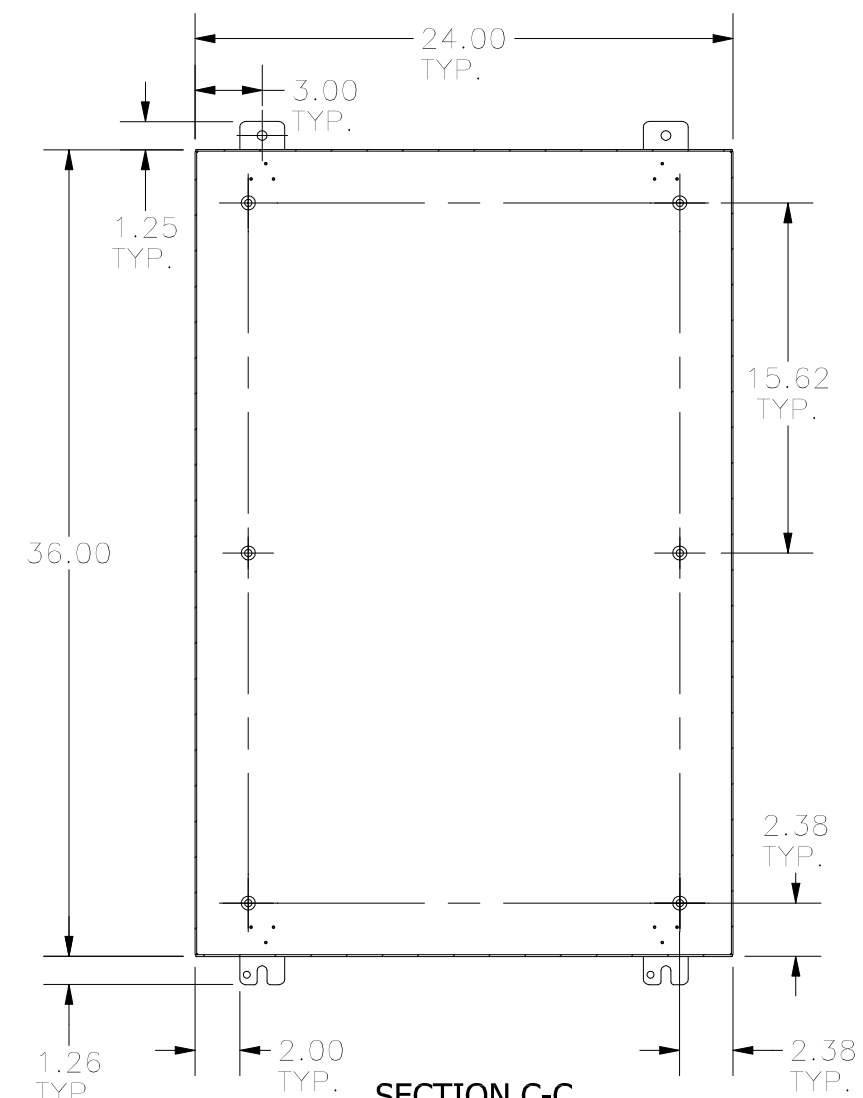
SECTION C-C BACK VIEW
