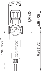
Semi auto Drain ** minimum clearance required to remove bowl
