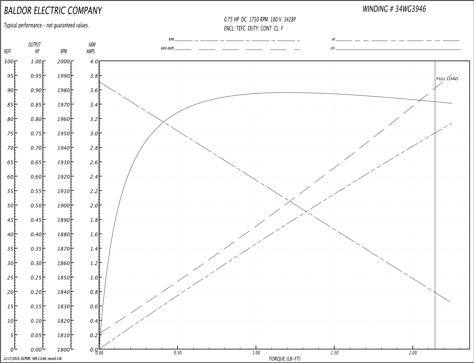
Performance Graph at 180.0 Arm V, 0.75HP Typical performance - Not guaranteed values
