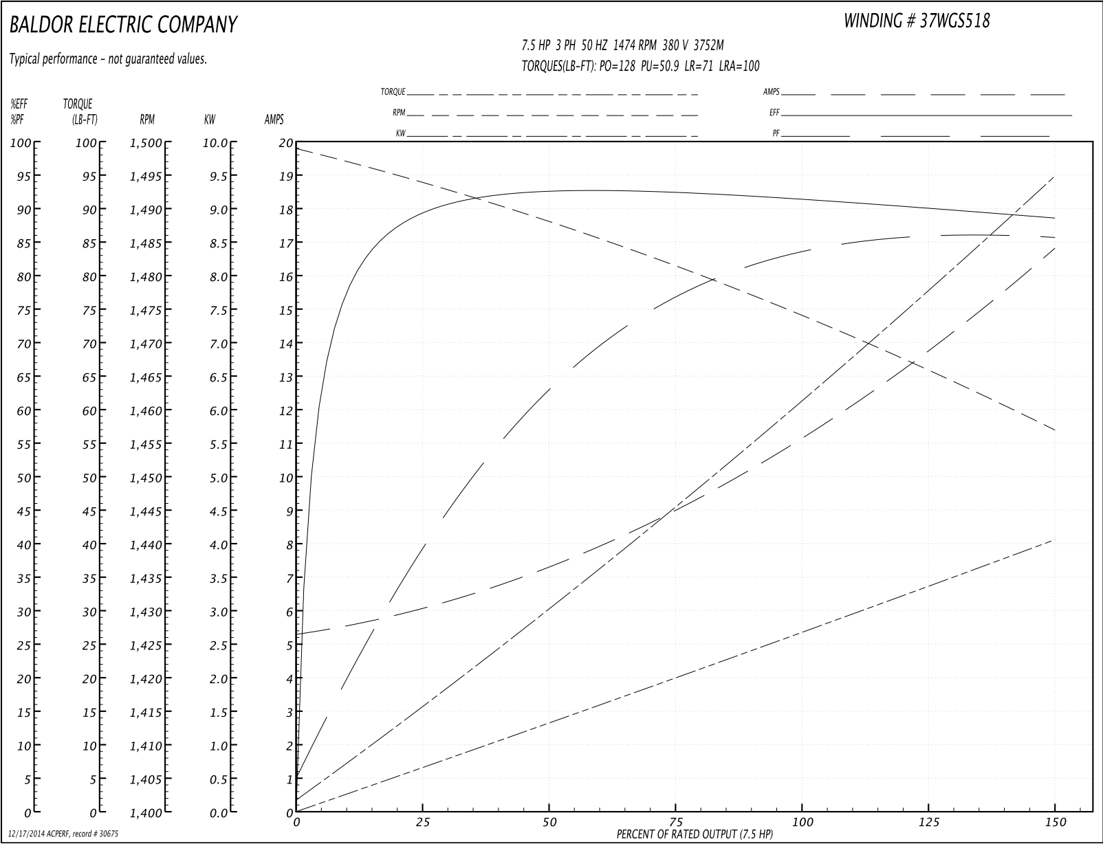
Performance Graph at 380V, 50Hz, 7.5HP Typical performance - Not guaranteed values
