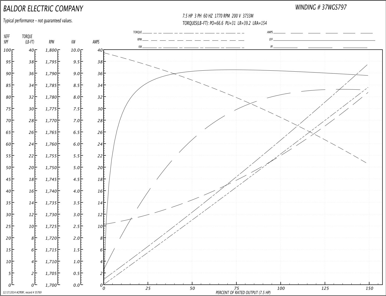
Performance Graph at 200V, 60Hz, 7.5HP Typical performance - Not guaranteed values
