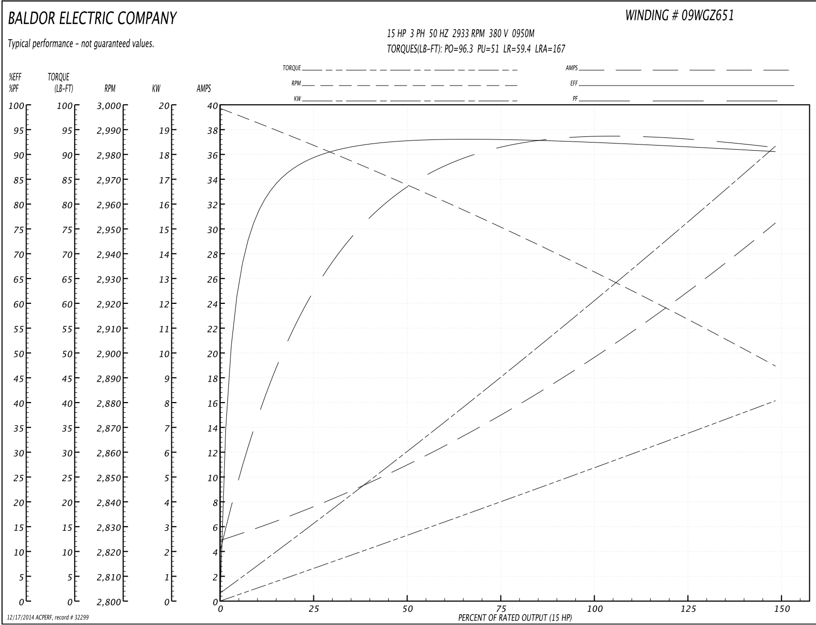
Performance Graph at 380V, 50Hz, 15.0HP Typical performance - Not guaranteed values
