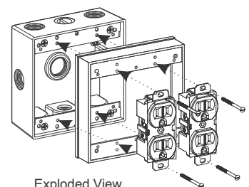
Exploded View, EXR-2 Shown Installed
