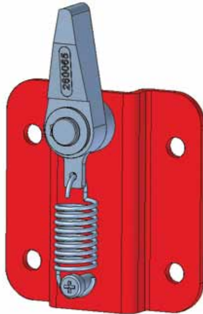
THE BELOW PICTURE SHOWS THE NEW DESIGN FOR THE LATCH MOUNTING BRACKET ASSEMBLY; 600643-XX SHOWN IN RED (AFTER MAY 2012)
