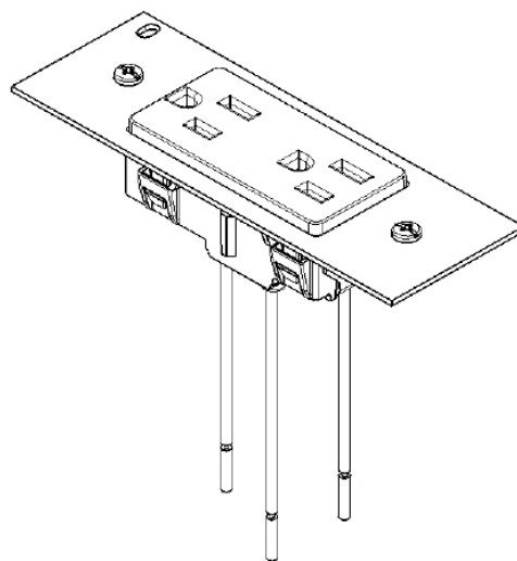
Leaded receptacle with faceplate Catalog No. PWFB10MPxxxx series PWFBMPDR15 example shown
