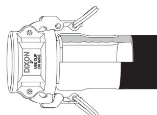
swaged assembly
