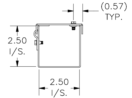
RIGHT VIEW
