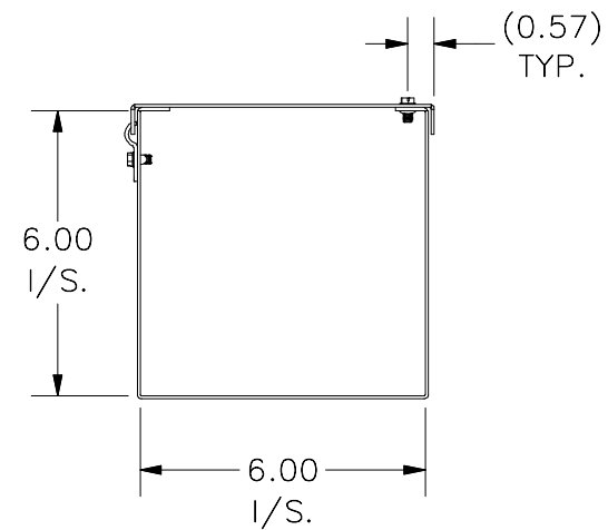
RIGHT VIEW
