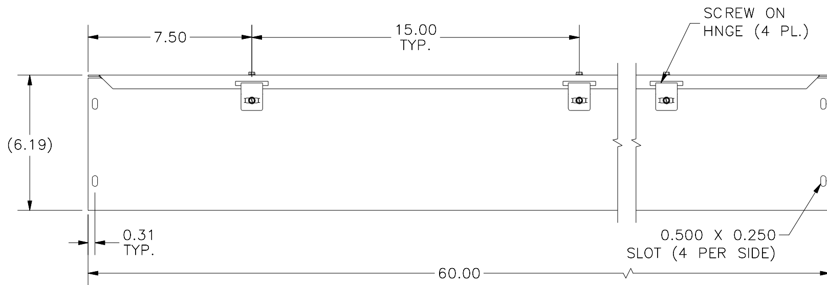
FRONT VIEW
