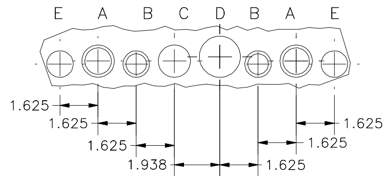
DETAIL A (8 PL. PER SIDE) K.O. PATTERN DESCRIPTION
