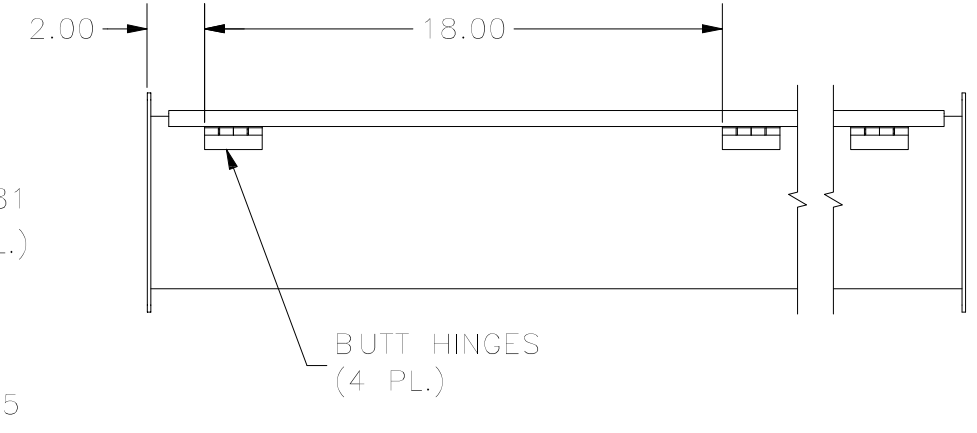
BACK VIEW
