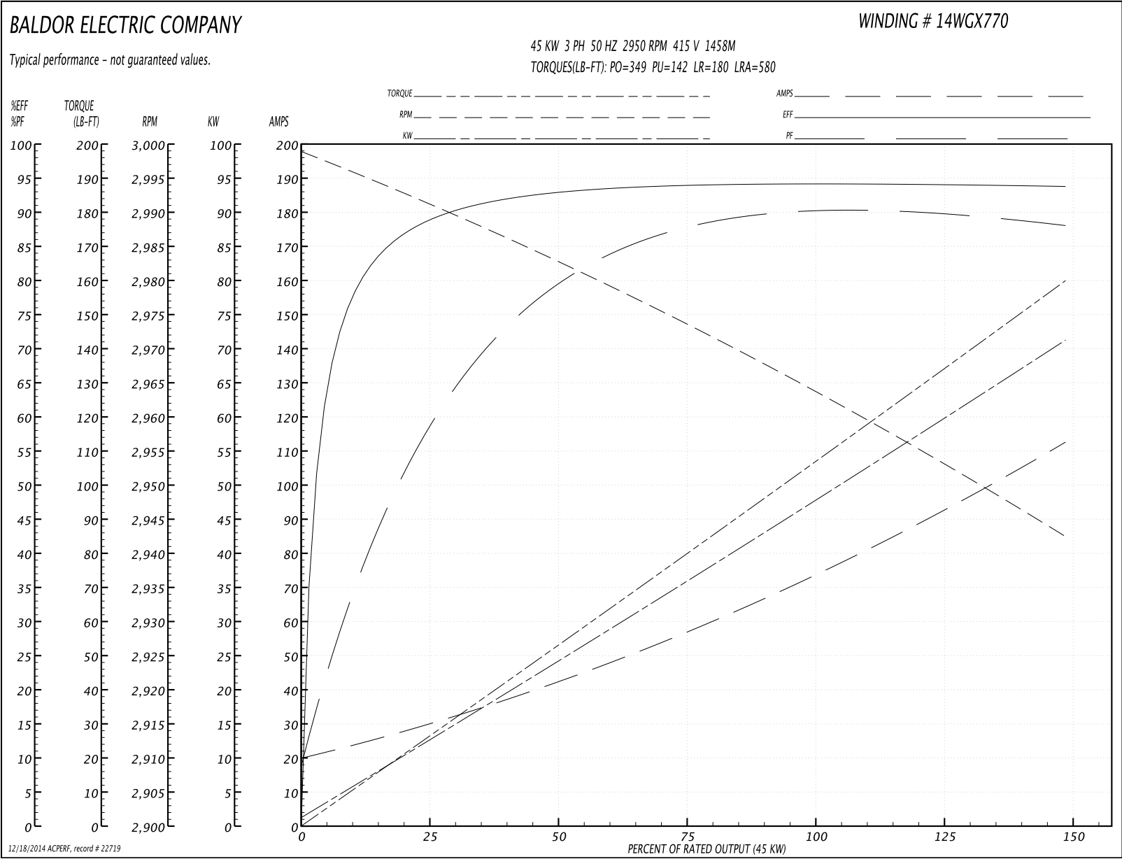
Performance Graph at 415V, 50Hz, 45.0KW Typical performance - Not guaranteed values
