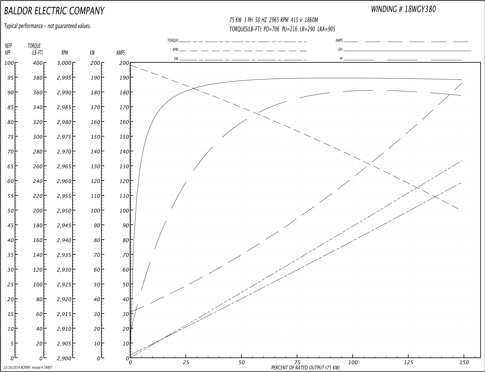
Performance Graph at 415V, 50Hz, 75.0KW Typical performance - Not guaranteed values
