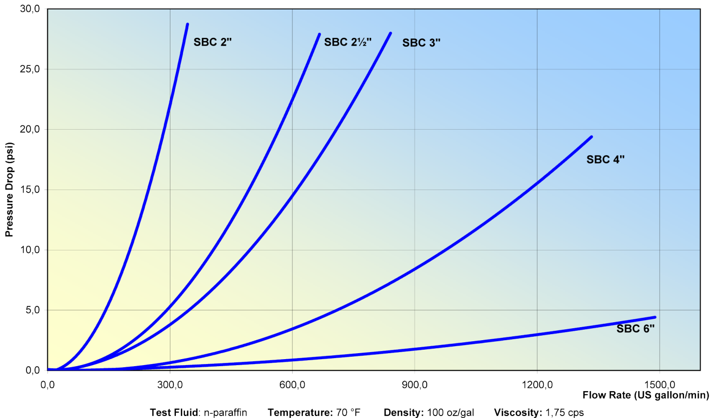
Flow Diagram (pressure drop)
