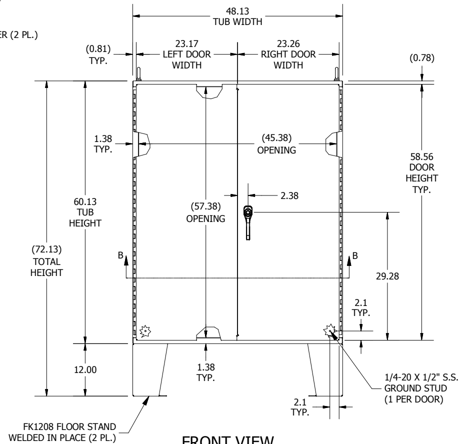
FRONT VIEW
