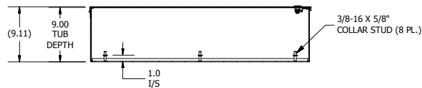
SECTION A-A (INSIDE TOP OF ENCL.)
