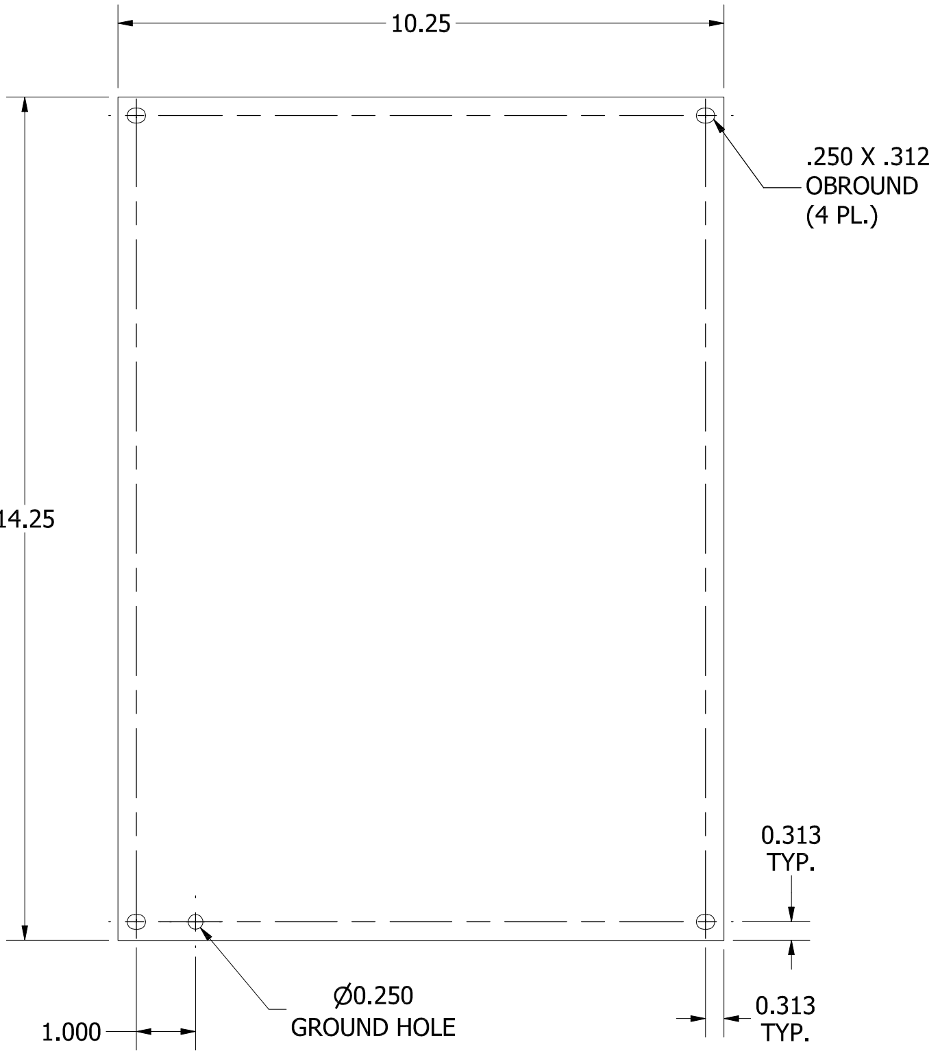
FRONT VIEW
