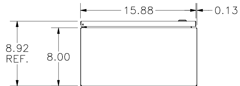
BOTTOM VIEW
