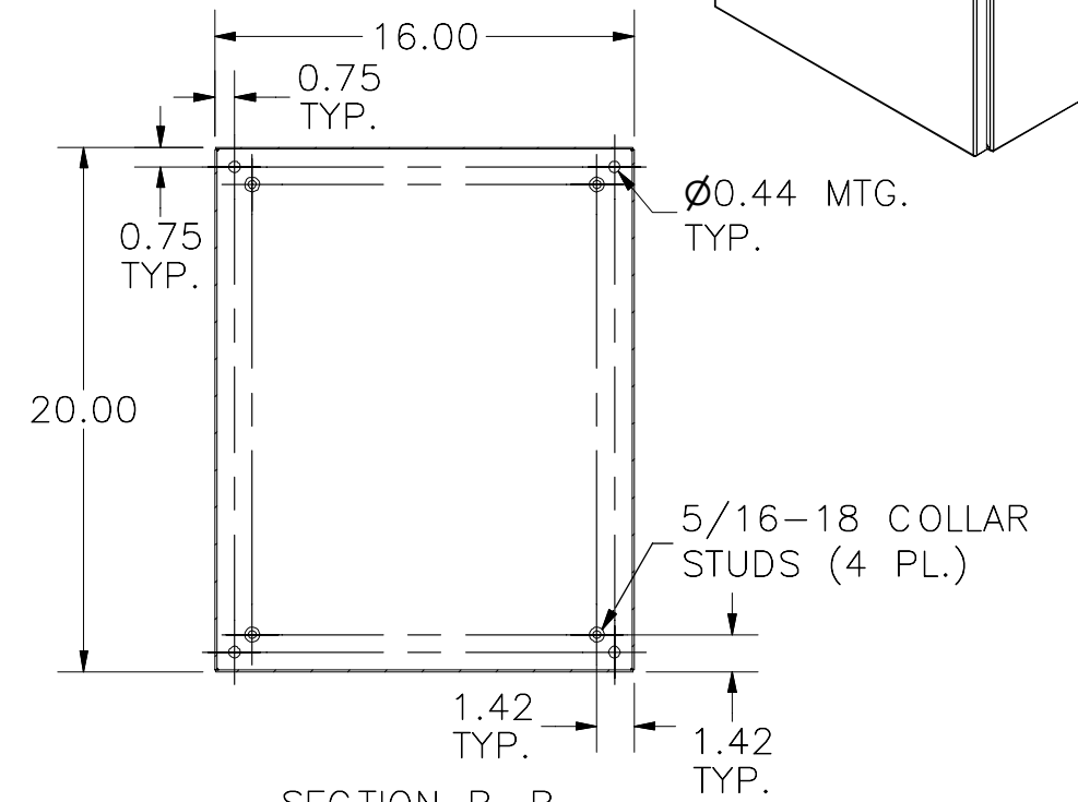
SECTION B-B (INSIDE BACK OF ENCLOSURE)
