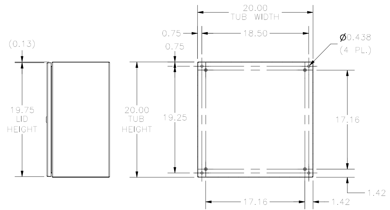
SECTION W-W (INSIDE BACK OF ENCLOSURE)
