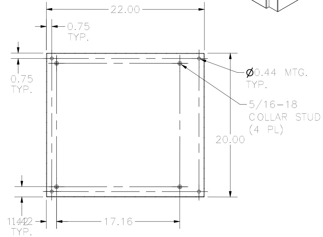
SECTION C-C (INSIDE BACK OF ENCLOSURE)
