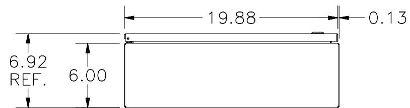
BOTTOM VIEW
