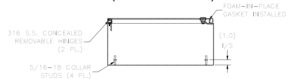
SECTION B-B VIEW (INSIDE TOP OF ENCL.)
