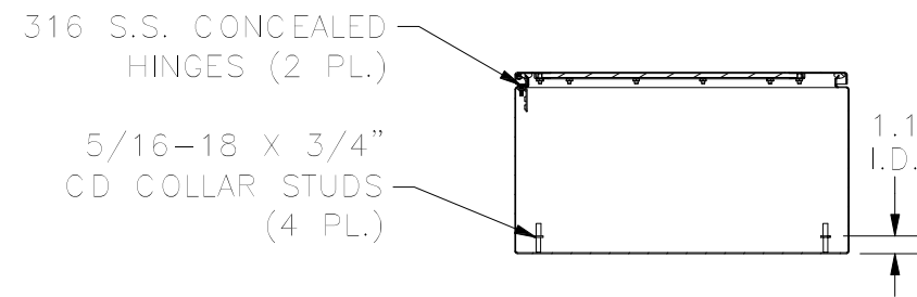
SECTION Y-Y (INSIDE BACK OF ENCLOSURE)
