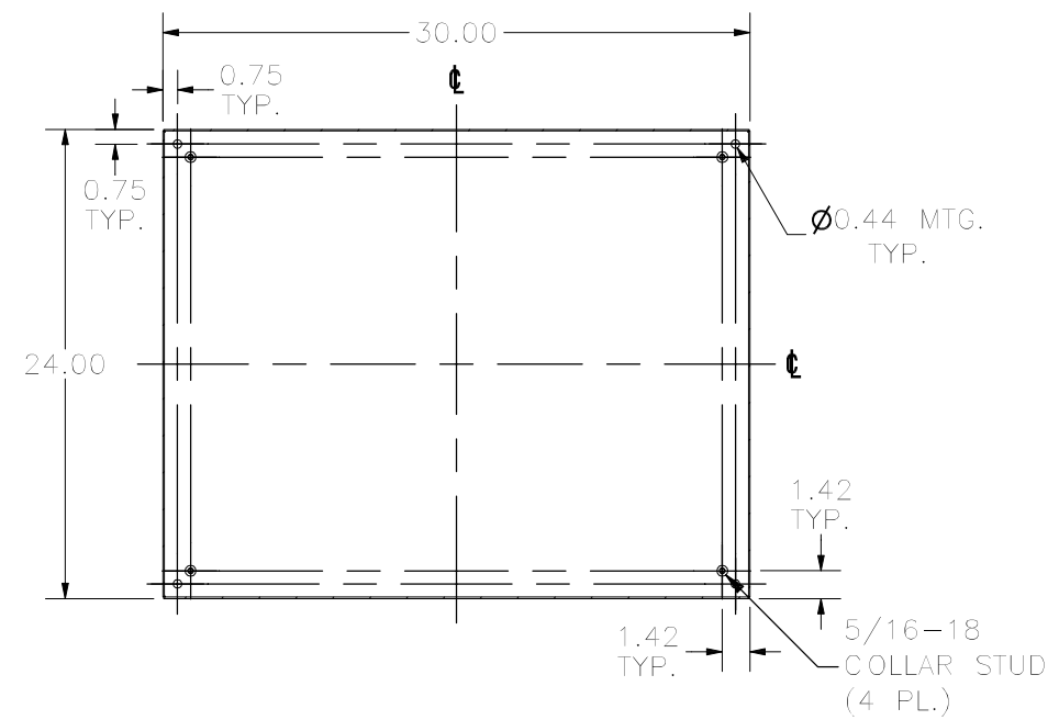
SECTION D-D VIEW (INSIDE BACK OF ENCLOSURE)
