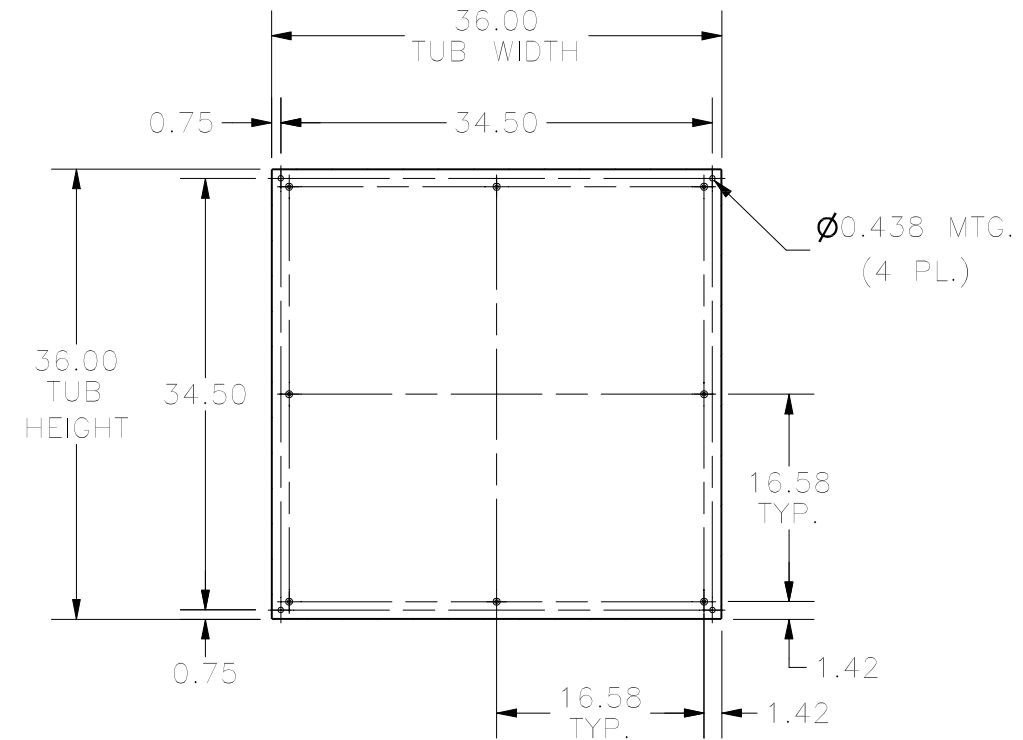
SECTION Y-Y (INSIDE BACK OF ENCLOSURE)
