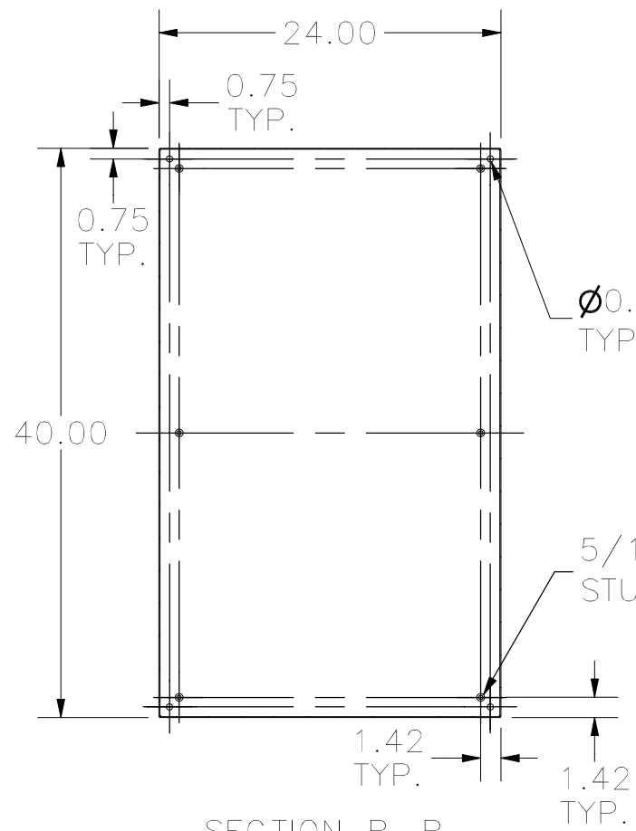
SECTION B-B (INSIDE BACK OF ENCLOSURE)
