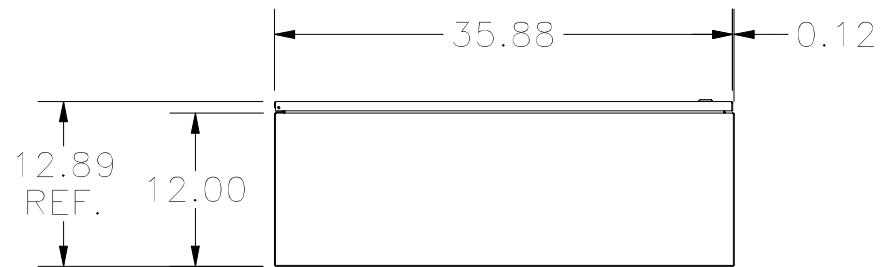
BOTTOM VIEW
