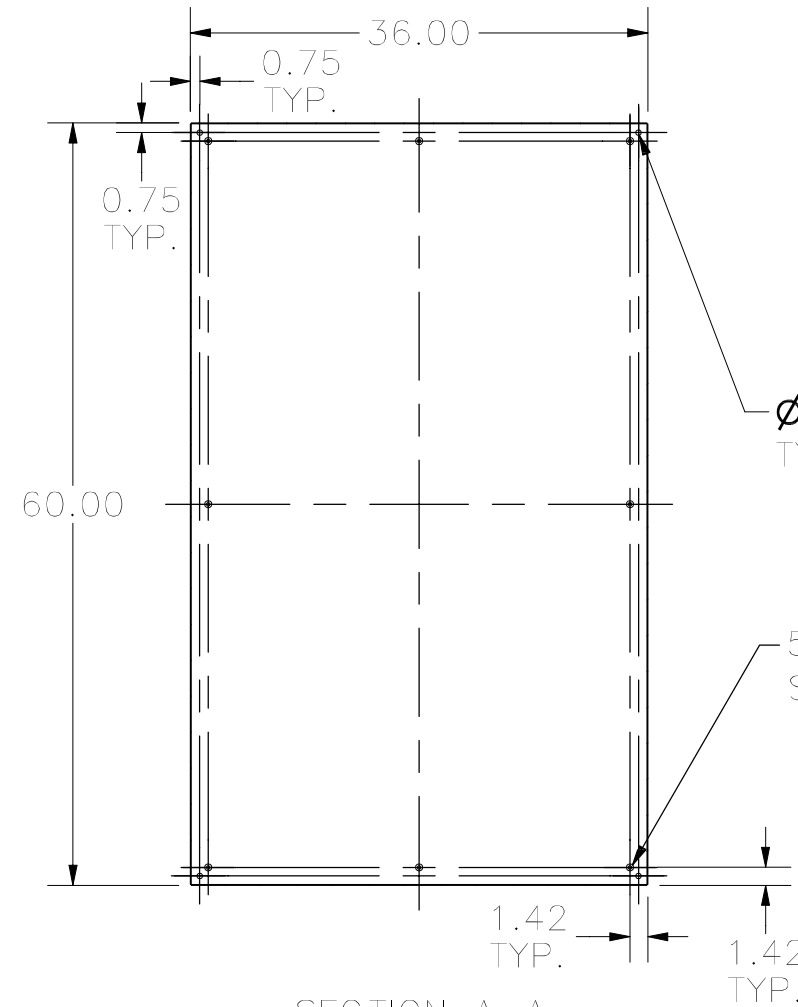
SECTION A-A (INSIDE BACK OF ENCLOSURE)
