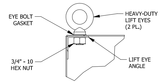
DETAIL AD (LIFT EYE ASSEMBLY VIEW)
