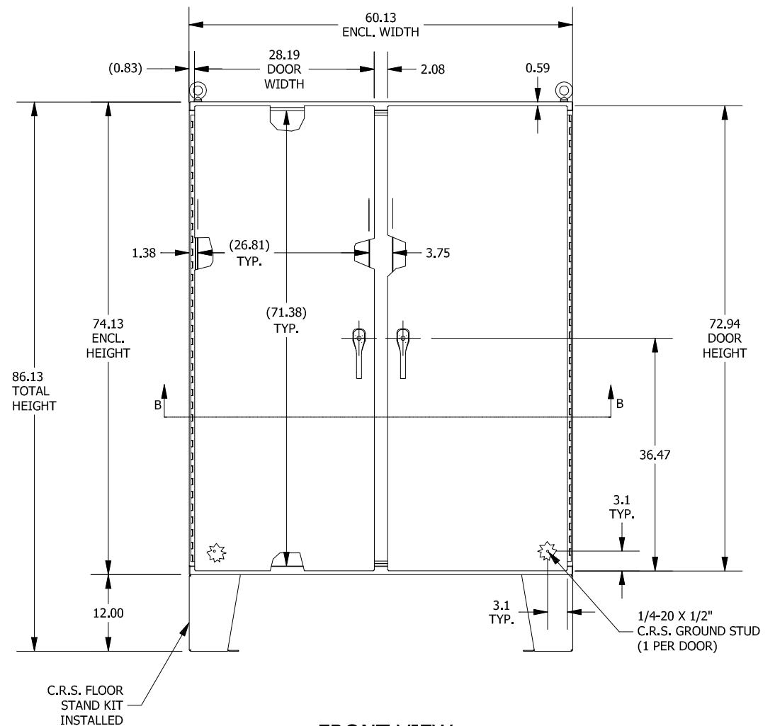
FRONT VIEW
