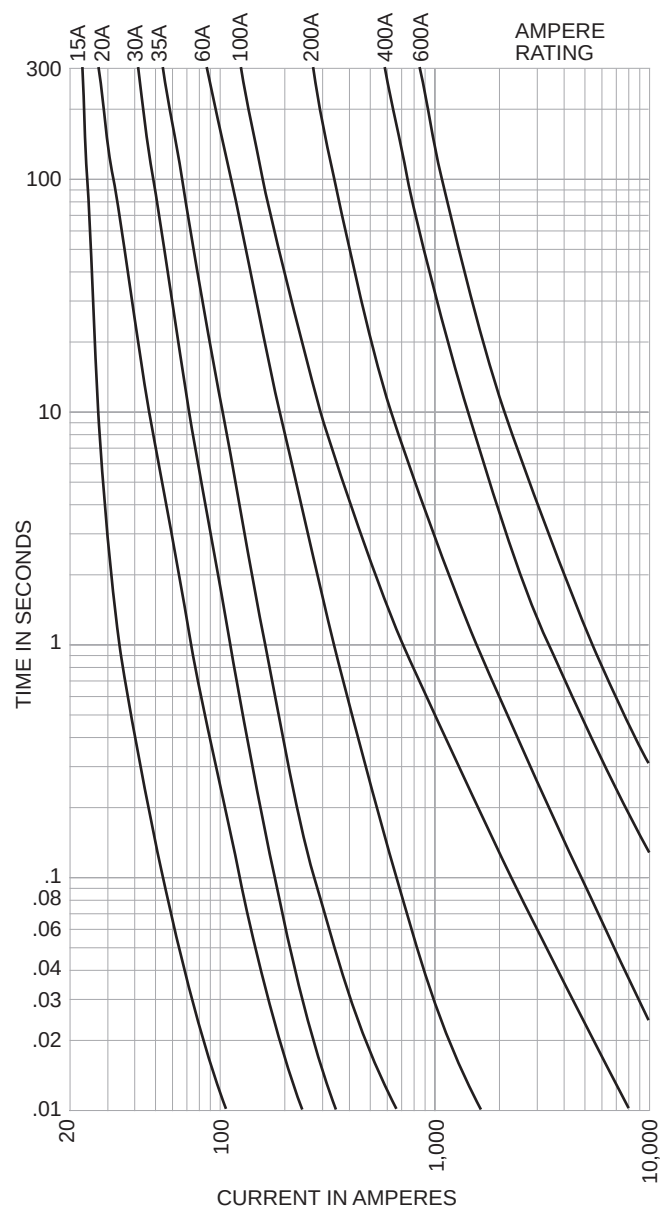
Time-Current Characteristic Curves—Average Melt NON ONE-TIME (250Vac) NOS ONE-TIME (600Vac)
