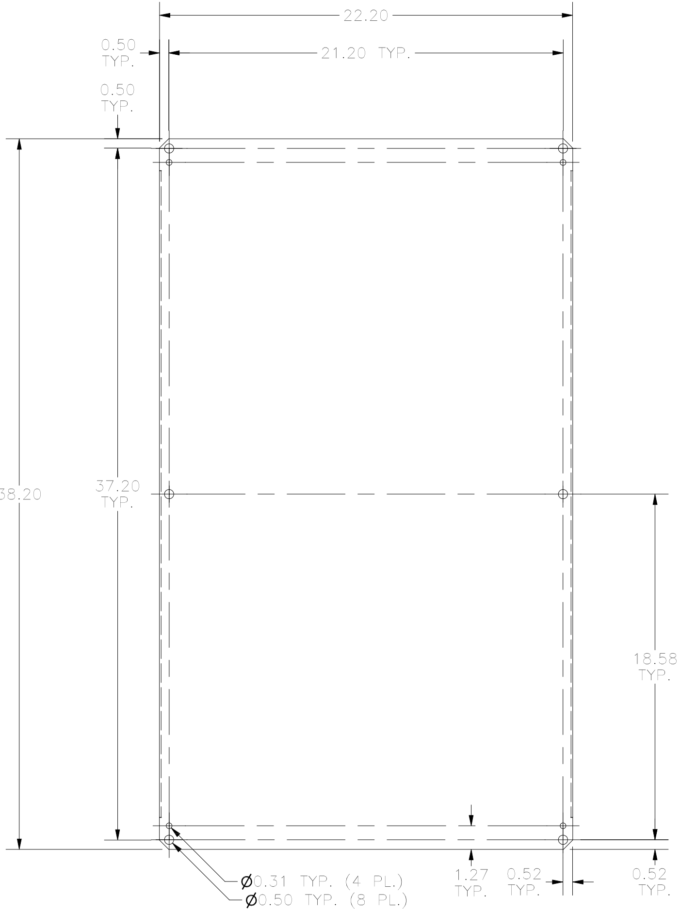
FRONT VIEW
