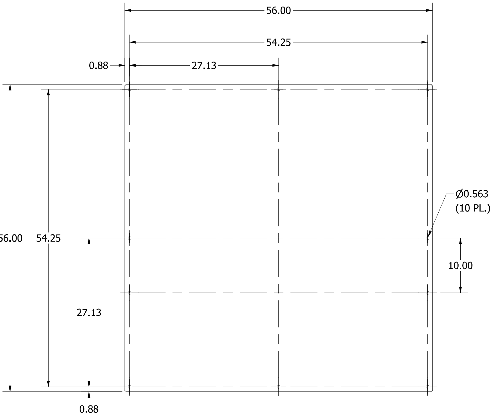
FRONT VIEW
