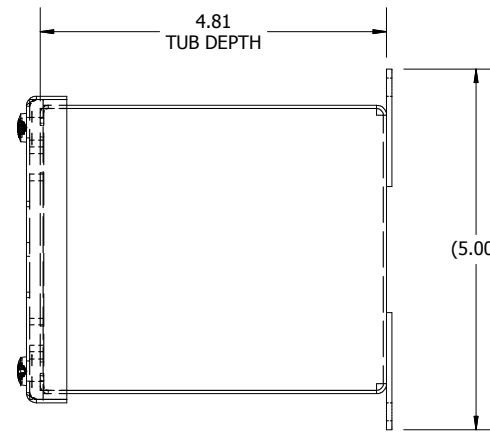
RIGHT VIEW
