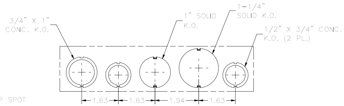
DETAIL C (KNOCKOUT DETAIL)
