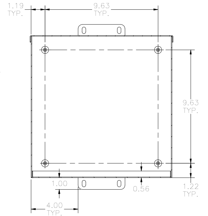
SECTION B-B VIEW (INSIDE BACK OF ENCL.)
