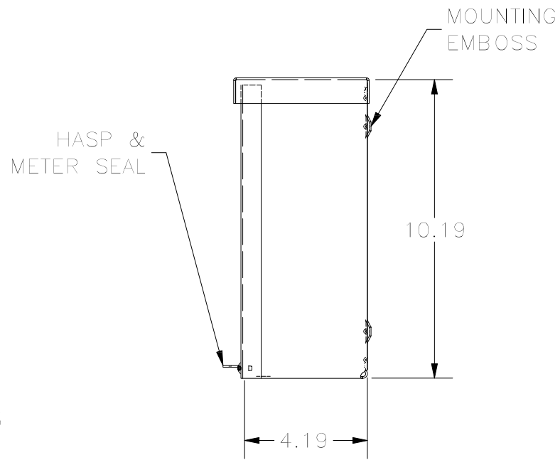
RIGHT VIEW
