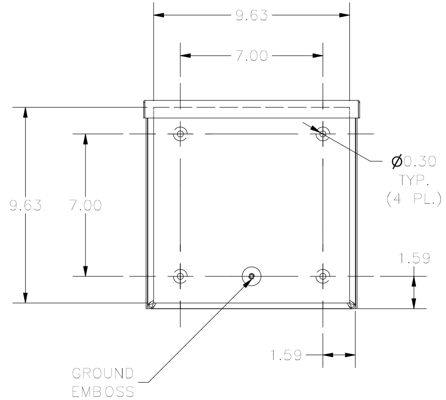
BACK VIEW
