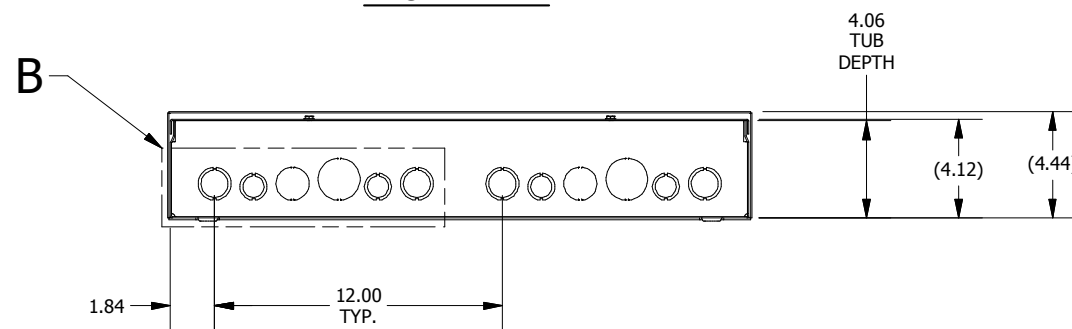
BOTTOM VIEW
