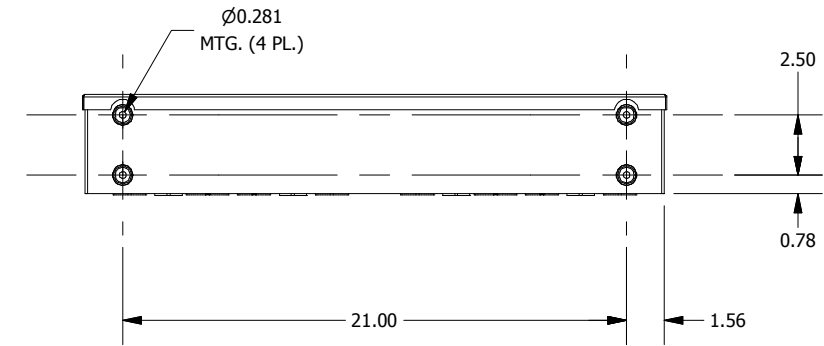
BACK VIEW
