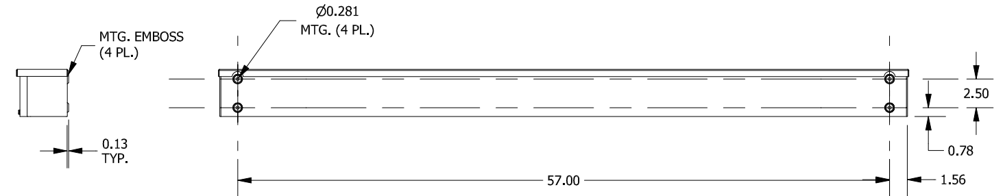
RIGHT SIDE VIEW
