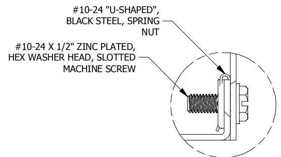
DETAIL A (3 PL.) (LID ATTACHMENT DETAIL)
