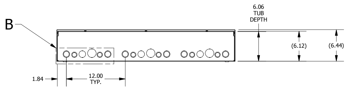
BOTTOM VIEW
