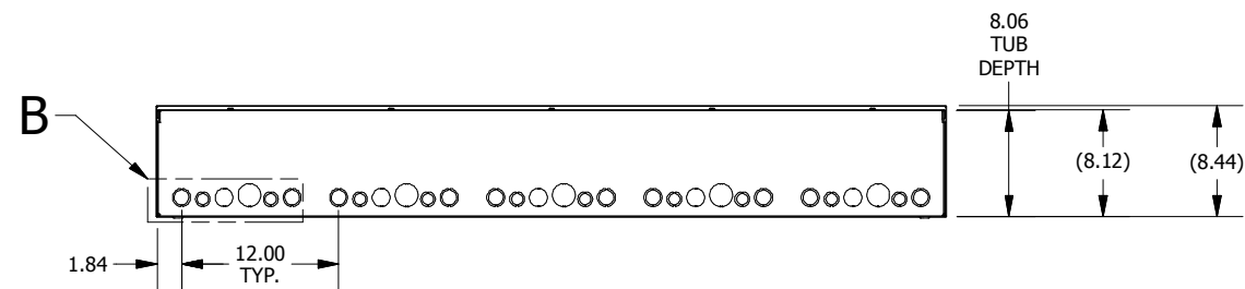
BOTTOM VIEW
