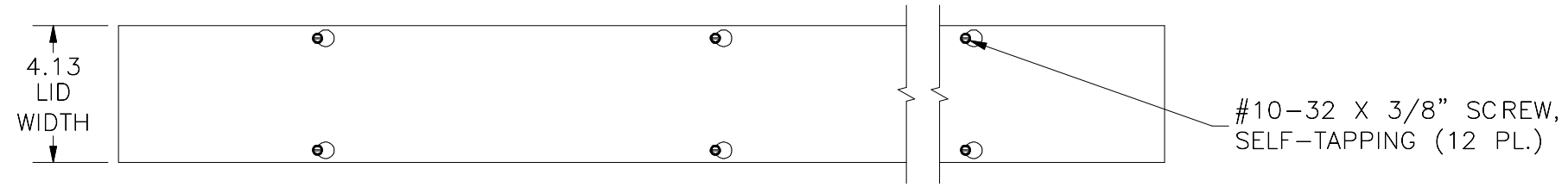
TOP VIEW
