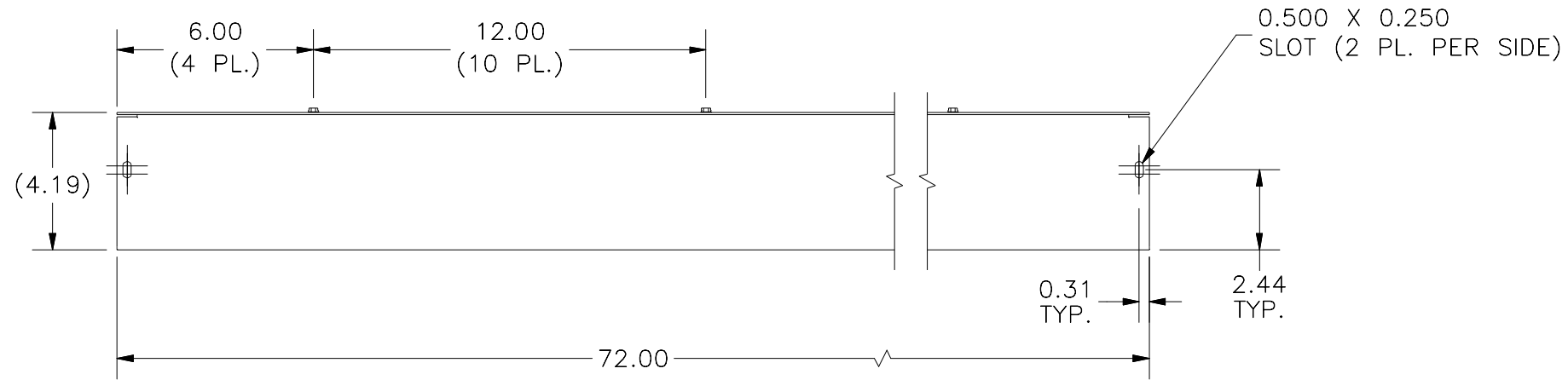
FRONT VIEW
