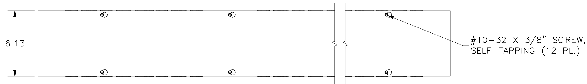
TOP VIEW
