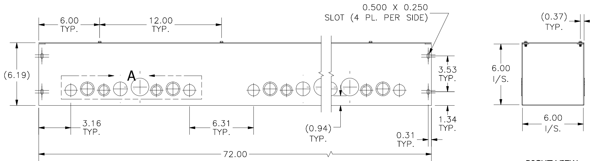
FRONT VIEW
