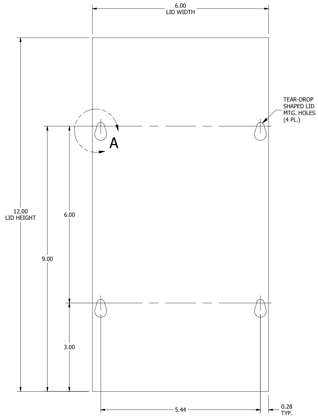
FRONT VIEW
