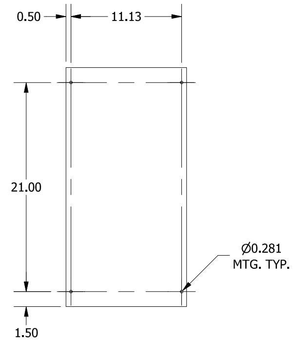
BACK VIEW
