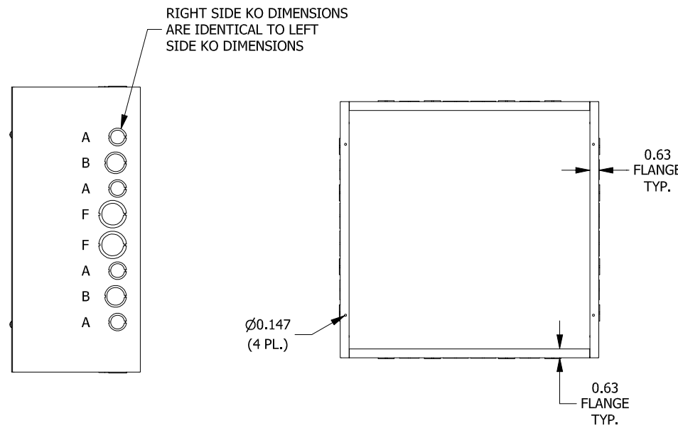
FRONT VIEW LID REMOVED
