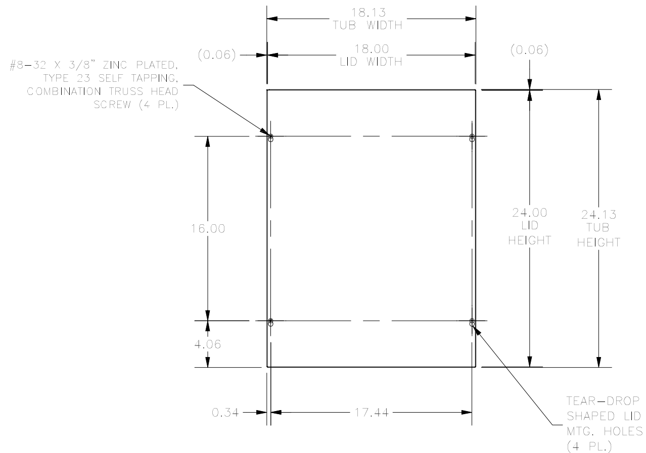
FRONT VIEW
