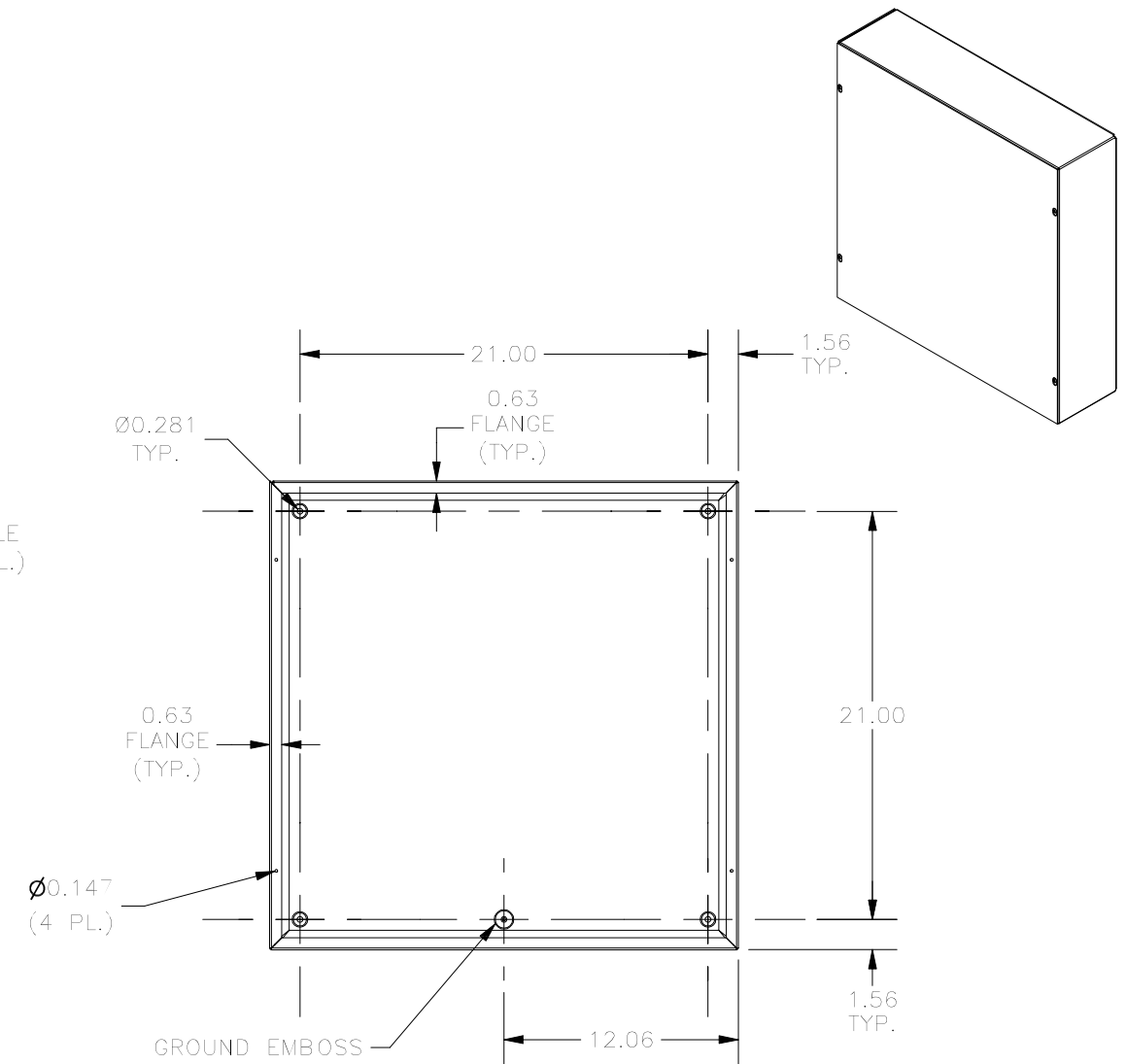
FRONT VIEW LID REMOVED
