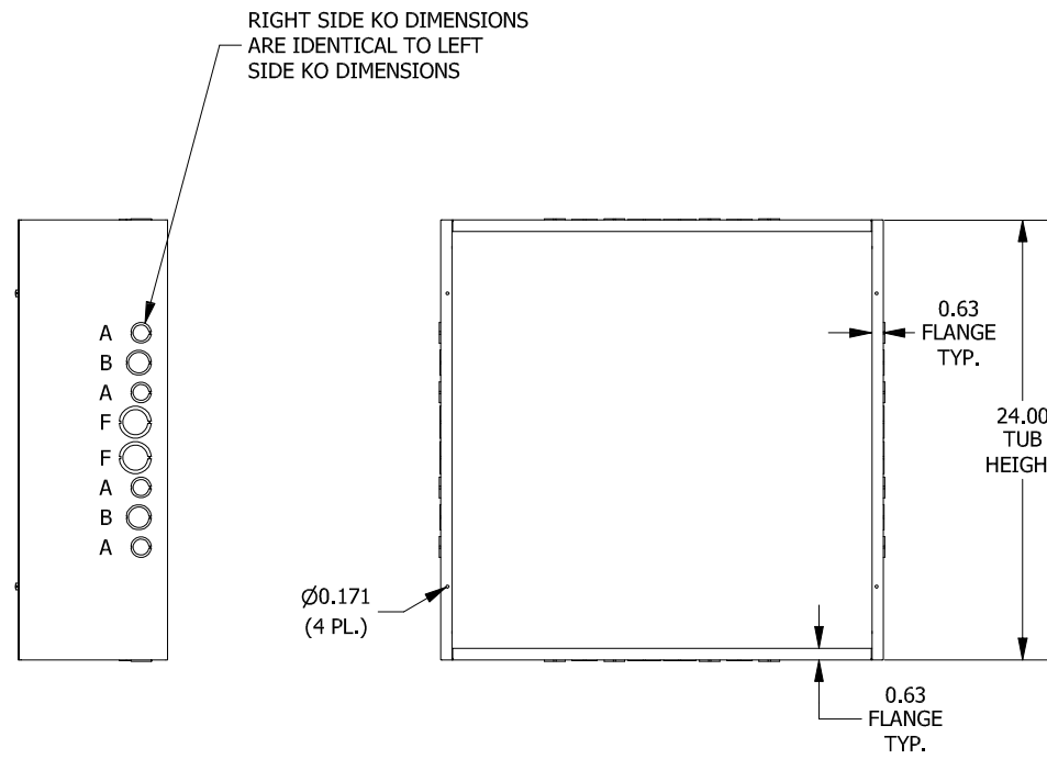
DETAIL A
